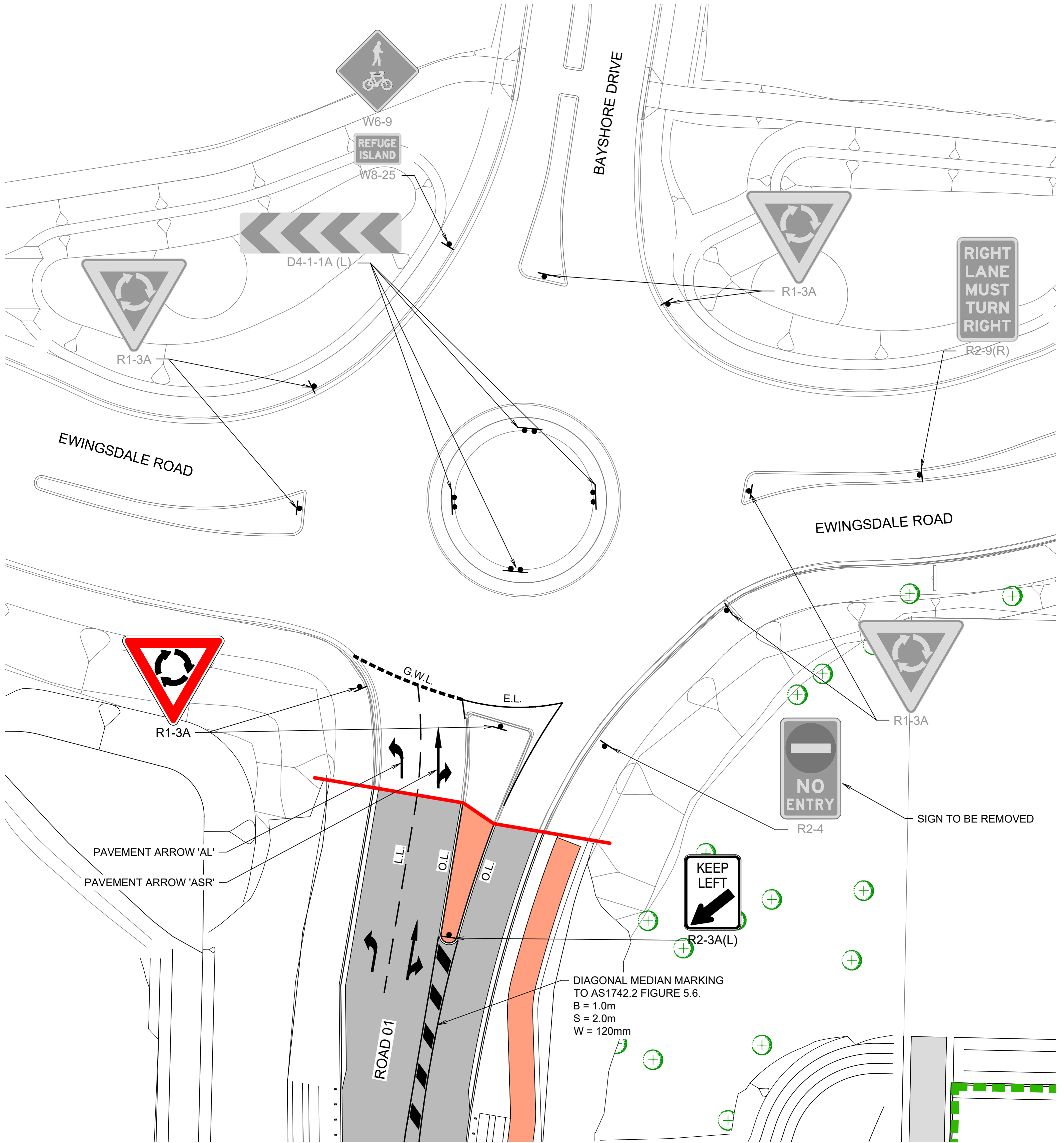
DETAIL C - ROUNDABOUT SIGNAGE AND LINEMARKING SCALE 1:250
