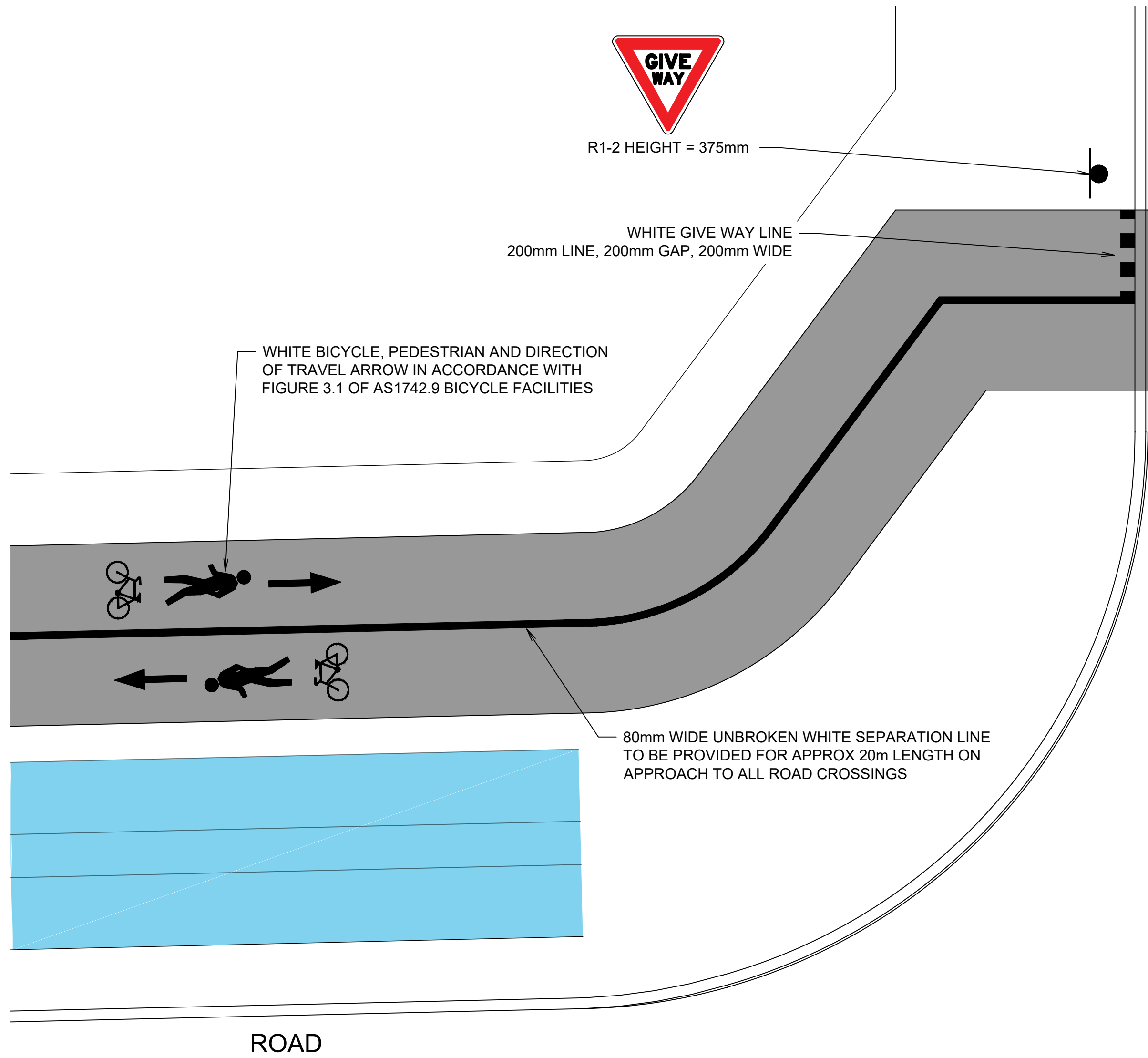
DETAIL A - TYPICAL PATH SIGNAGE AND LINEMARKING SCALE 1:50
